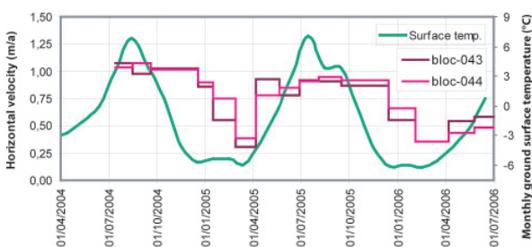
Figure 4: Seasonal variations of horizontal velocities [m a -1 ] (Juno4-Julo6) of boulders 43 and 44 placed on the front of L2 and ground surface temperature (°C).
