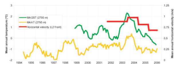
Figure 2: Comparison between MAGST [°C] MAAT [°C] and mean annual velocities [m a -1 ] on front of L2.
