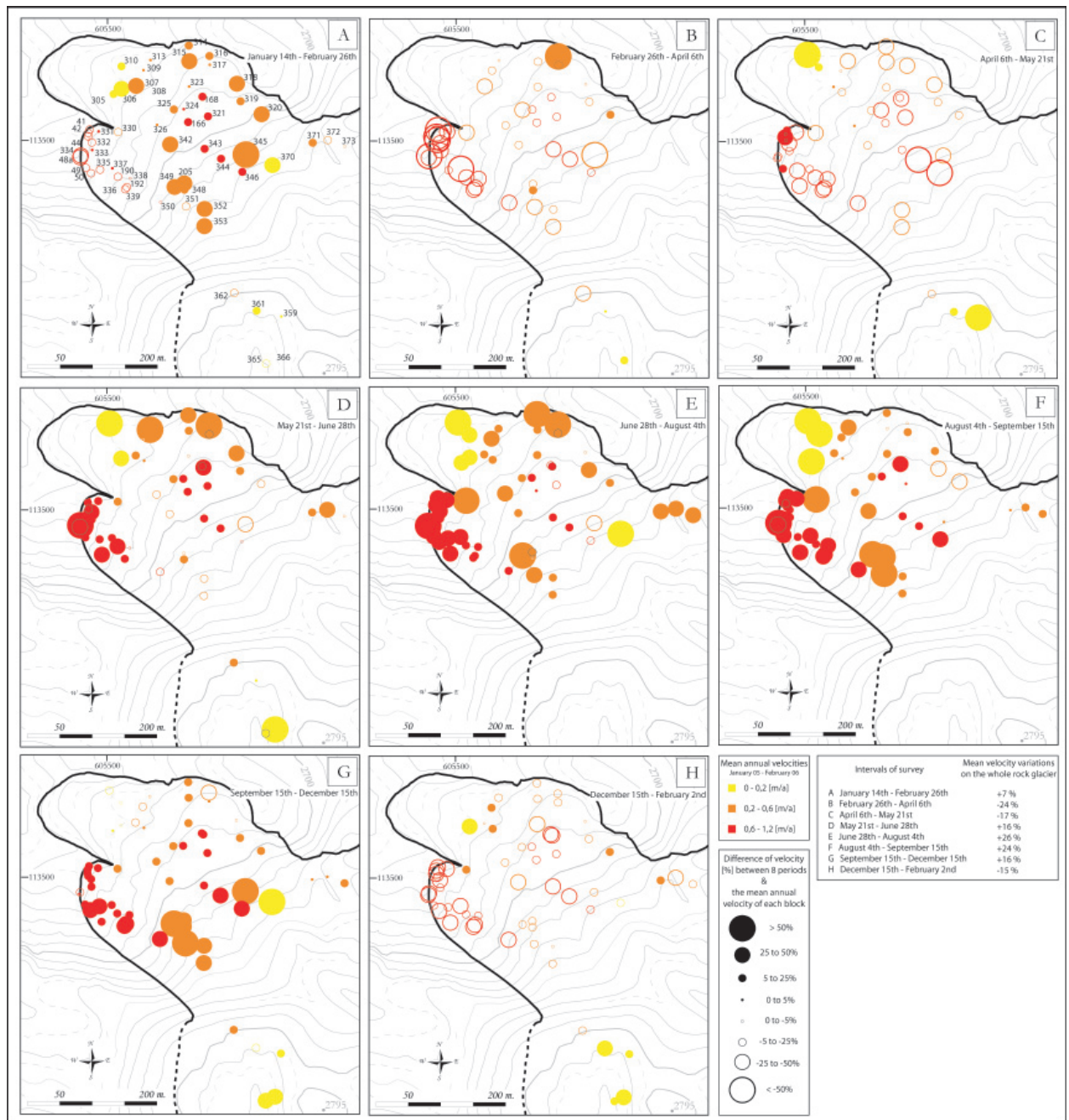
Figure 5: Mean annual horizontal velocities (Jan. 05 – Feb. 06) for ~60 boulders on BBRg and “seasonal” velocity variation [in % compared to the annual mean]. For phases A-H, see comments in text.
