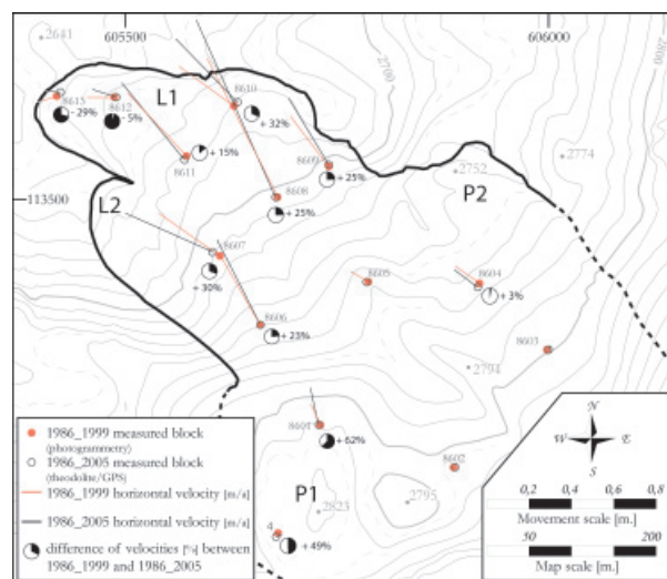
Figure 1: Mean annual horizontal movement [m a -1 ] on BBrg for the time period 1986-1999 (photogrammetry) and 1986-2005 (theodolite-GPS). Dots show the initial position of “photogrammetric” and “geodetic” boulders used for comparison (they may be different).
