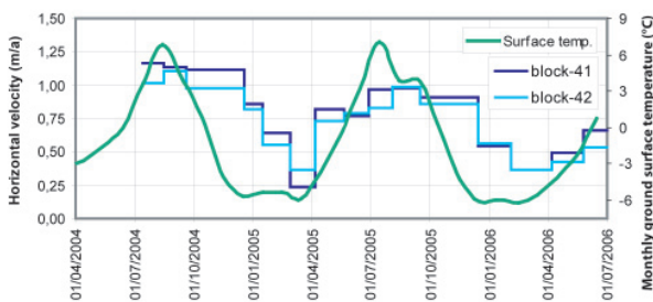
Figure 3: Seasonal variations of horizontal velocities [m a -1 ] (Juno4-Julo6) of boulders 41 and 42 placed on the front of L2 and ground surface temperature (°C).
