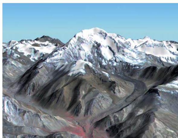
Figure 12: Glacier Surge of the Horcones Inferior glacier (left: photograph of 1/2006 by Deutscher/Hirschmugl; right: perspective view with ASTER data of 1/2004).
