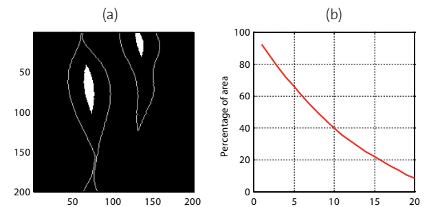
Figure 7: Snow cover on a flat surface and CA with neighborhood of Moore: (a) Remaining snow cover after 20 time units and T=6, (b) Dynamic behavior of the snow-cover.
