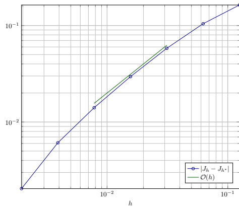
(a) functional value J_h
