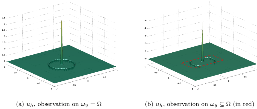
Fig. 6.2: Comparison of optimal controls u_h for full observation ( \omega_y = \Omega ) and partial observation ( \omega_y \subsetneq \Omega , marked in red).
