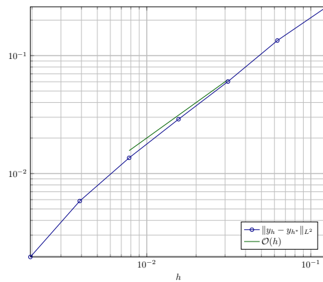
(b) L^2 norm of state y_h
