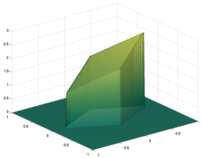
(a) target y_{d,1}
